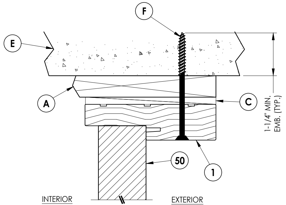
4 VERTICAL CROSS SECTION 7 Inswing Shown w/ 1X Buck
