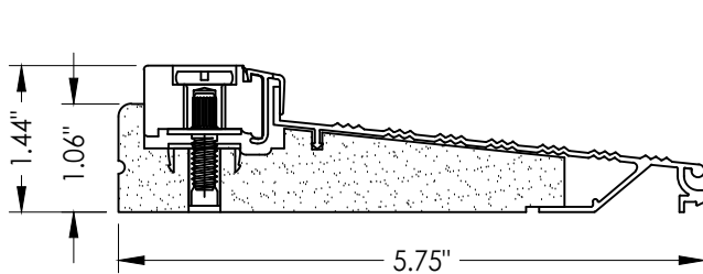
14 INSWING THRESHOLD Young Mfg.
