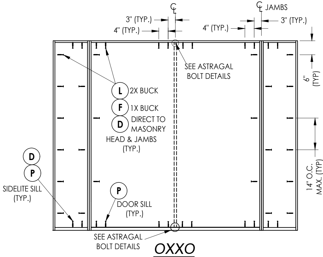
FRAME ANCHORING
