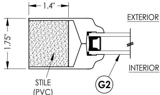
2 HORIZONTAL CROSS SECTION 3
