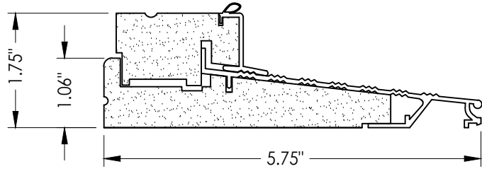
16 INSWING THRESHOLD w/ SIDELITE ADAPTER Young Mfg.
