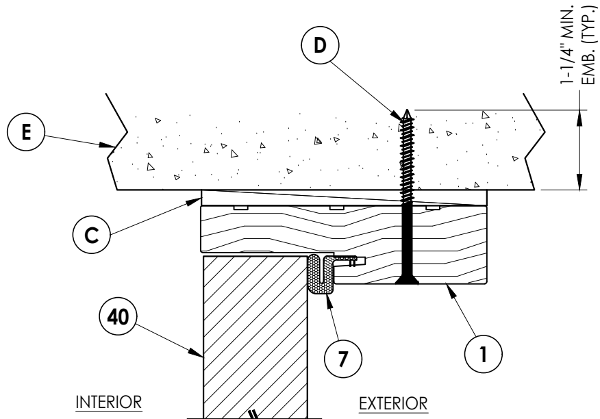
3 8 VERTICAL CROSS SECTION Inswing Shown Direct to Masonry
