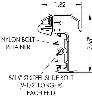
53 ENDURA ULTIMATE ALUMINUM ASTRAGAL ULTIMATE PUSH BUTTON ASTRAGAL
