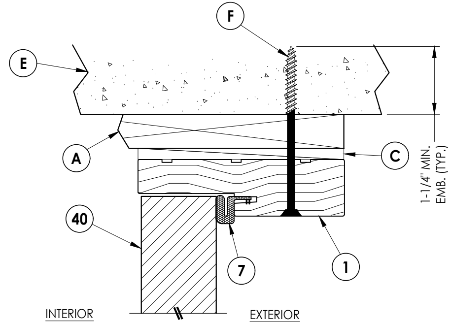
3 VERTICAL CROSS SECTION 7 Inswing Shown w/ 1X Buck
