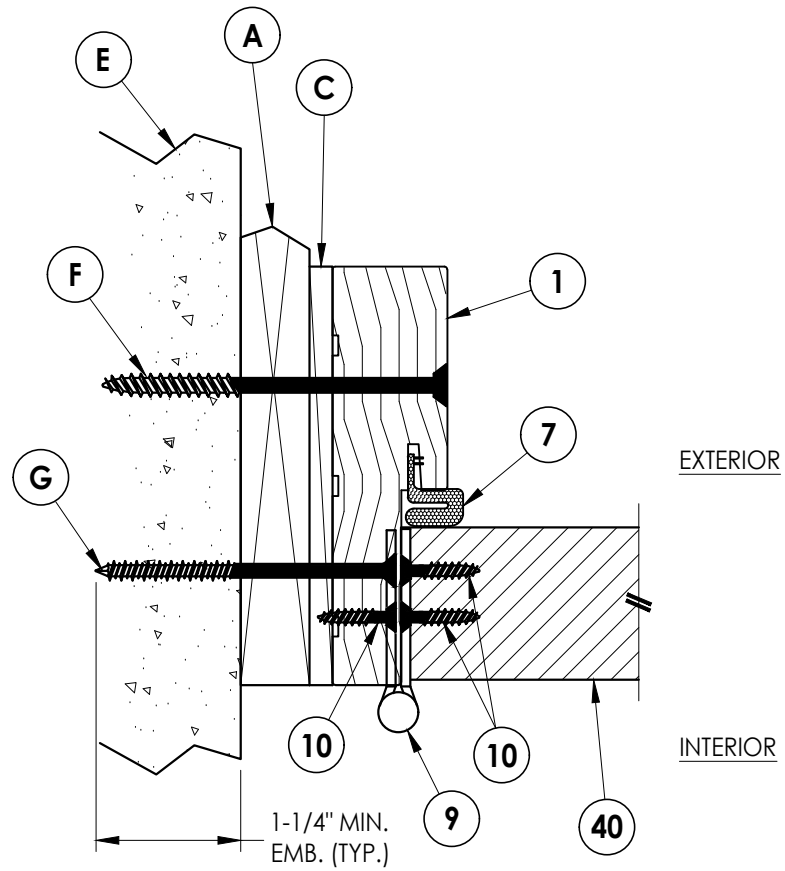
1 HORIZONTAL CROSS SECTION 7 Inswing Shown w/ 1X Buck
