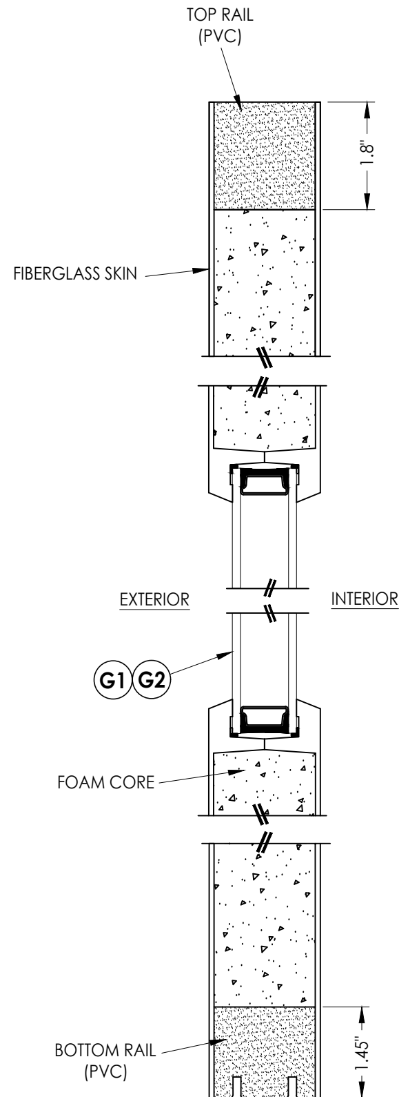
2 VERTICAL CROSS SECTION 3
