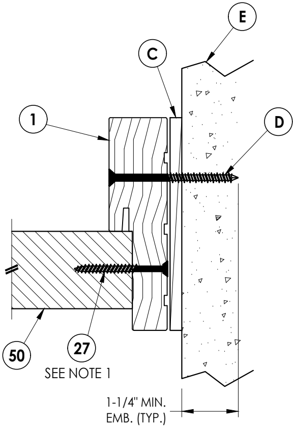
2 8 HORIZONTAL CROSS SECTION Inswing Shown Direct to Masonry
