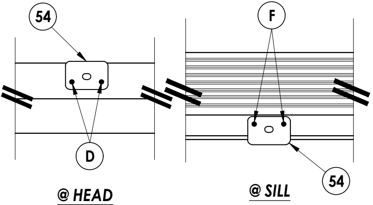
ASTRAGAL BOLT STRIKE DETAIL
